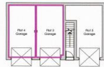
GROUND FLOOR PLAN (GARAGES) Scale 1:200 @ A2
